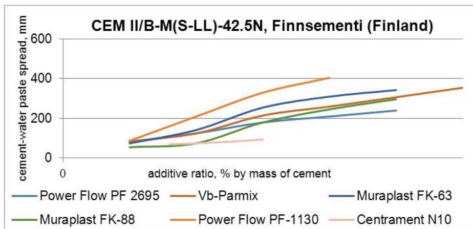
Figure 5. The results of tests of additives with CEM II/B-M(S-LL)-42.5N, Finnsementi
