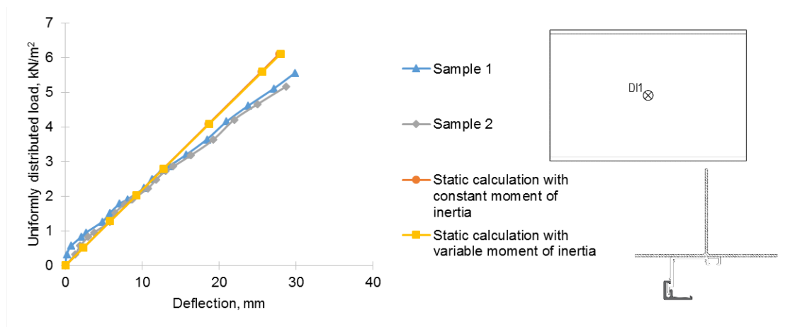
Figure 19. Deflection of the center of the panel (DI1).
