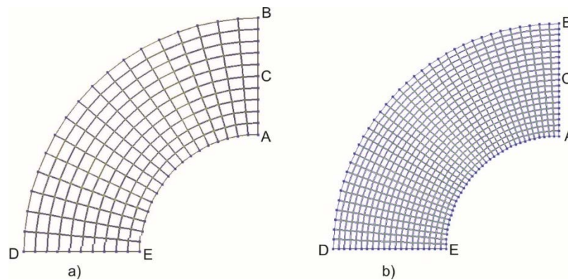
Figure 4. Finite-element meshes of the half-ring.
