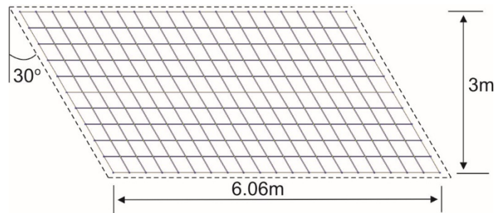
Figure 3. The skew plate with hinge supports.
