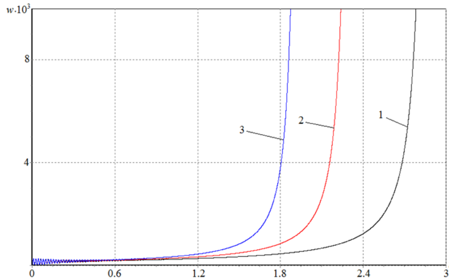
Figure 5. Dependence of the deflection on time for various values of the velocities of loading 1 – P_0 = 2 \text{ MPa/s} ; 2 – P_0 = 2.5 \text{ MPa/s} ; 3 – P_0 = 3 \text{ MPa/s} .
