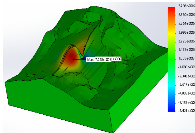
Figure 17. The form 4 of natural oscillations of the dam for the spatial problem.
