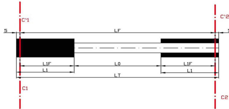
Figure 3. Length of the GFRP bars.
